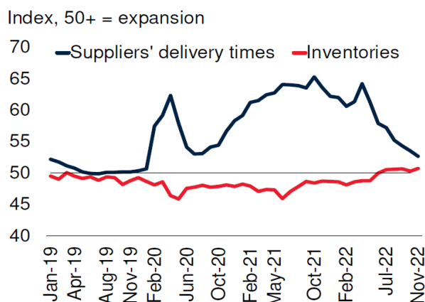
Figure 1.2.B - Manufacturing PMIs
